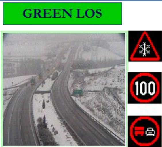
Figure 1.- Image of the road network with green level of service. On the right, the signals used in VMS.
