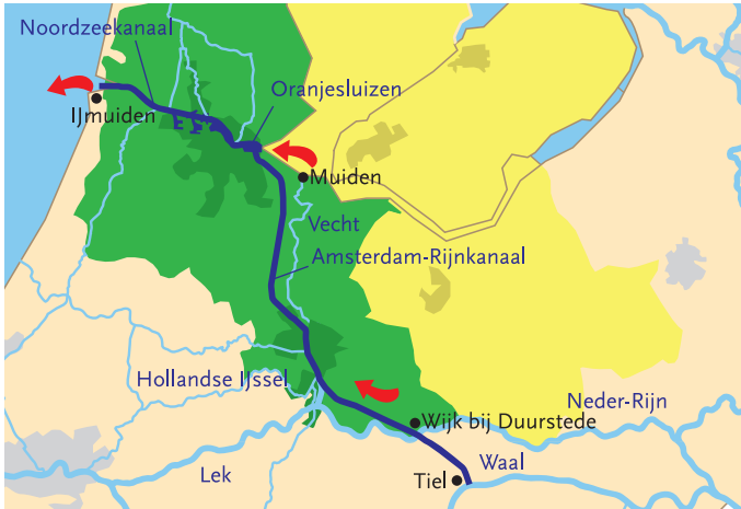
Catchment area of the subsystem of the Amsterdam-Rijnkanaal and Noordzeekanaal. Green drains directly, yellow indirectly.
