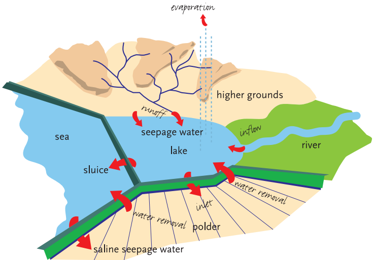
The interconnectedness of the water system components.
