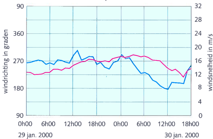
K13a platform
