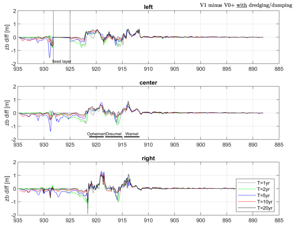
Figure 59 Bed level difference between V1 and V0 at left bank, centre of channel and right bank, whole model.
