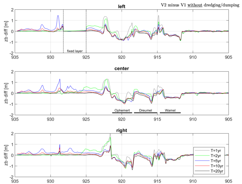
Figure 69 Bed level difference between V2 and V1 at left bank, centre of channel and right bank, LTW-area and downstream, simulation without dredging/dumping.
