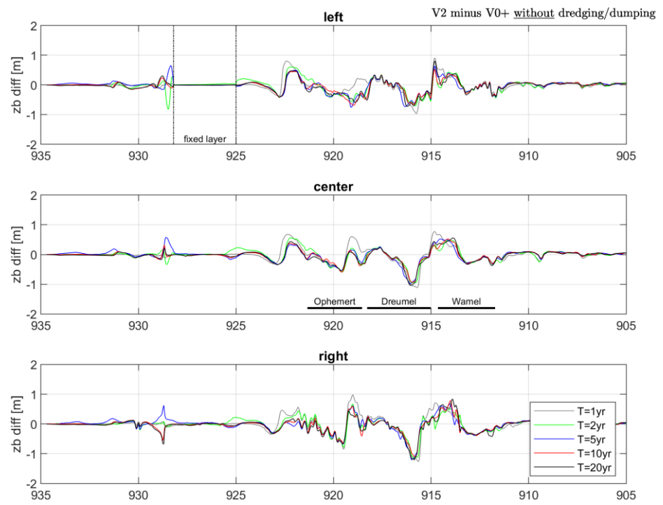
Figure 68 Bed level difference between V2 and V0 at left bank, centre of channel and right bank, LTW-area and downstream, simulation without dredging/dumping.
