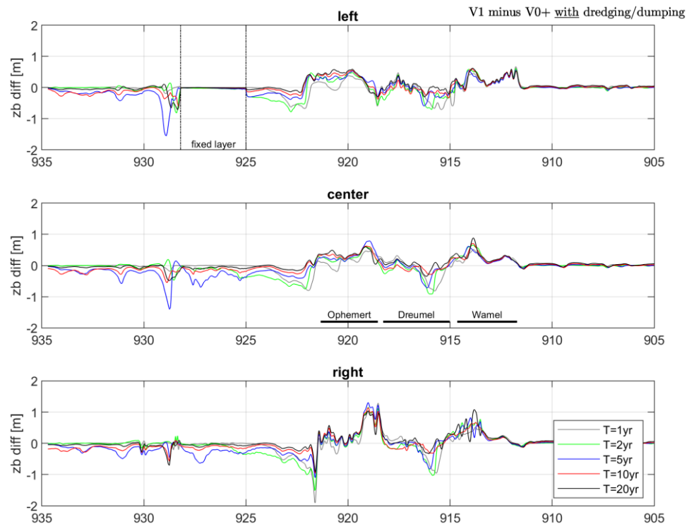
Figure 60 Bed level difference between V1 and V0 at left bank, centre of channel and right bank, LTW-area and downstream.
