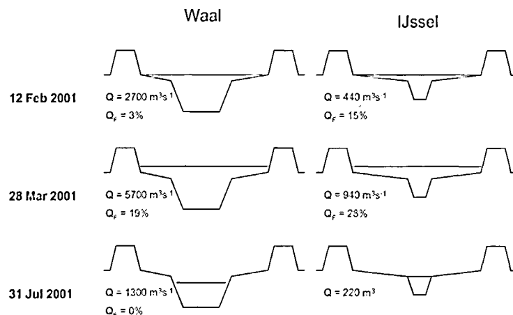
Figure 4. Cross sections of the rivers Waal and IJssel showing discharges ( Q ), as well as percentages of the discharge flowing through floodplains ( Q_F ), during the three sampling events. Arrows indicate sampling locations.
