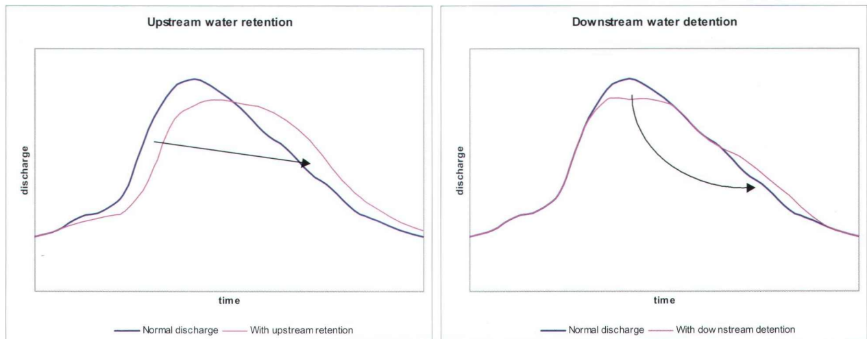
Figure 3. Theoretical change in hydrographs due to upstream water retention and downstream water detention, assuming enough storage space available.
