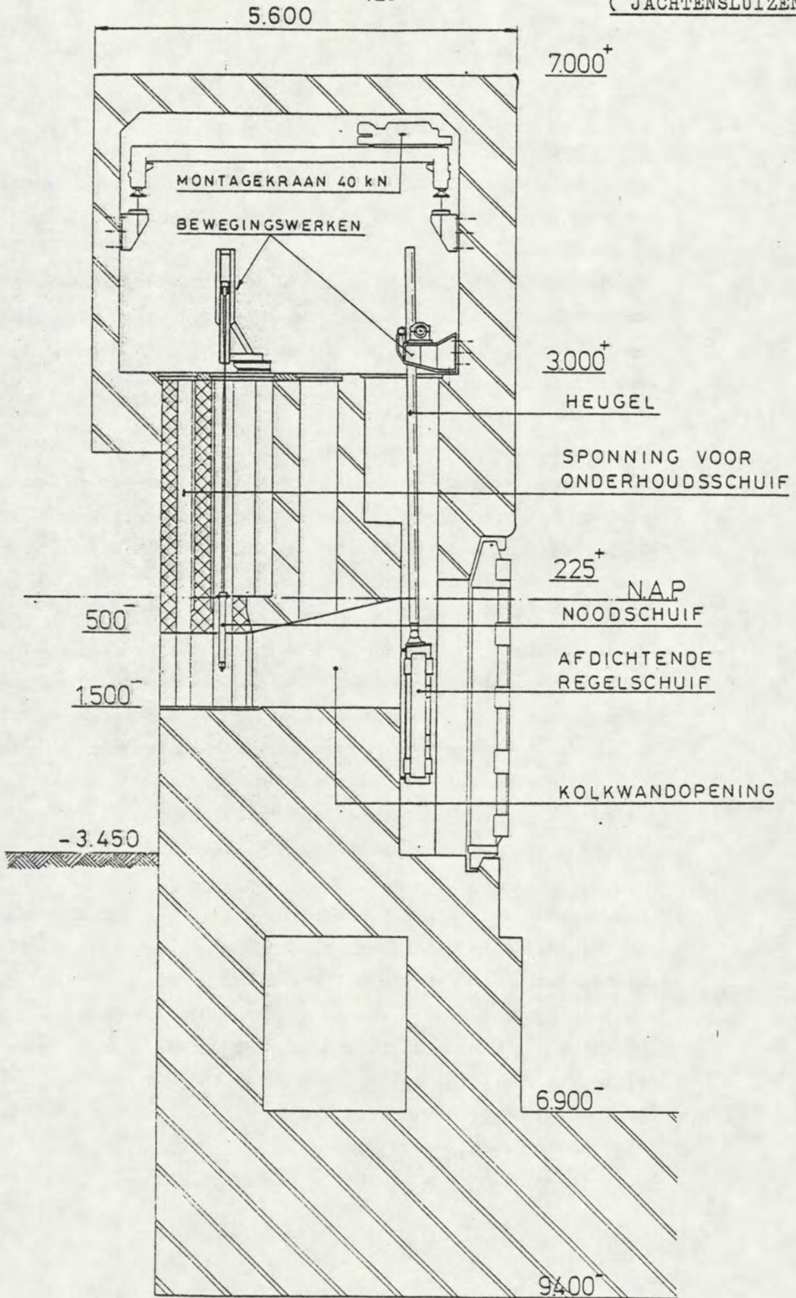
MATEN IN mm fig. 4.6
